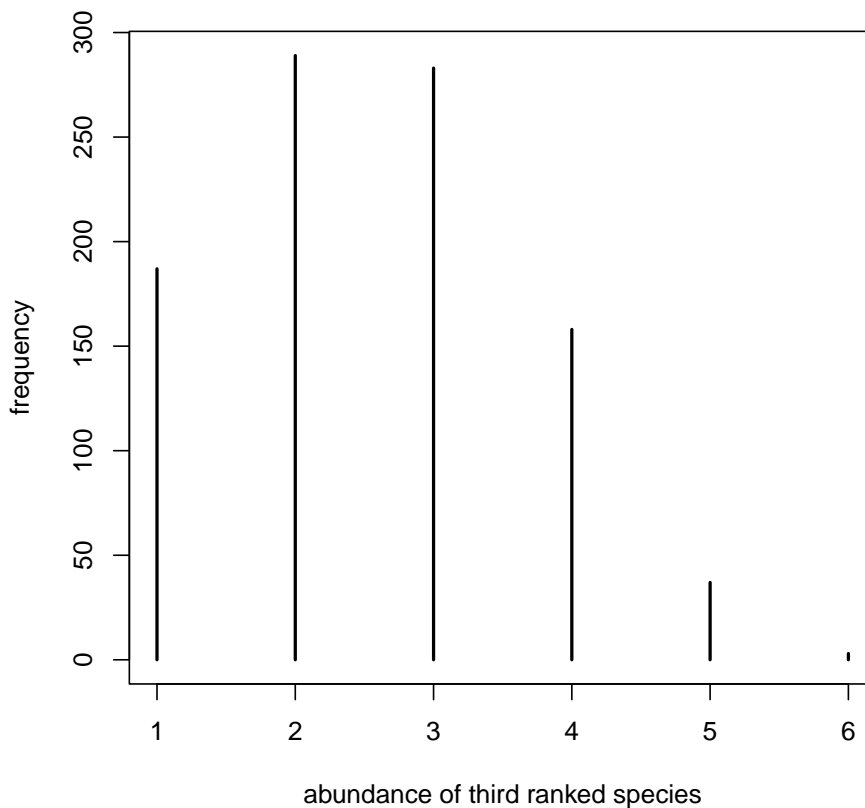
Figure 5: Abundance of third ranked species of an ecosystem of J_M = 20 individuals and a biodiversity parameter \theta = 2 : 1000 replicates
