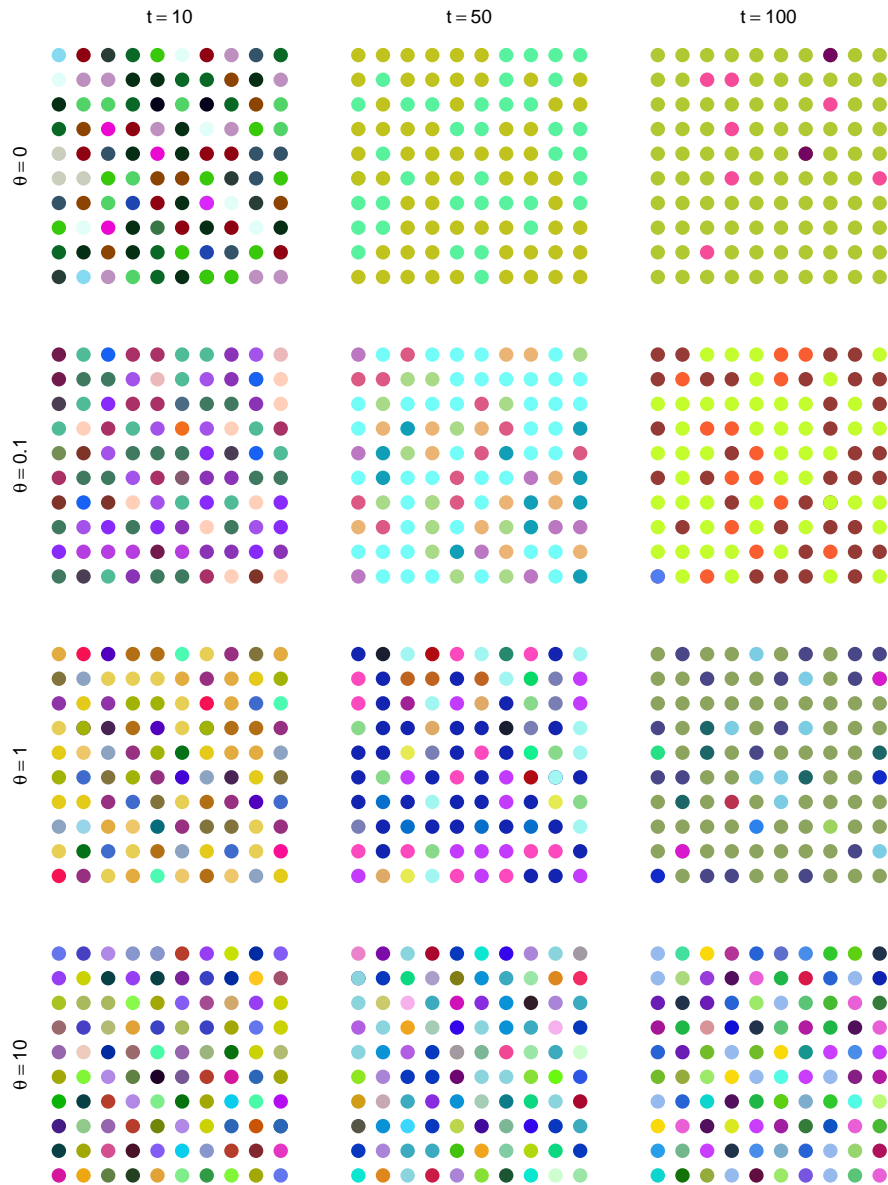
Figure 7: Simulated ecosystems of size J_M = 100 for varying parameters, with each organism represented by a dot, the different colours representing different species; spatial locations are functionally identical. Initial conditions are a system of maximal diversity (i.e. 100 singletons)
