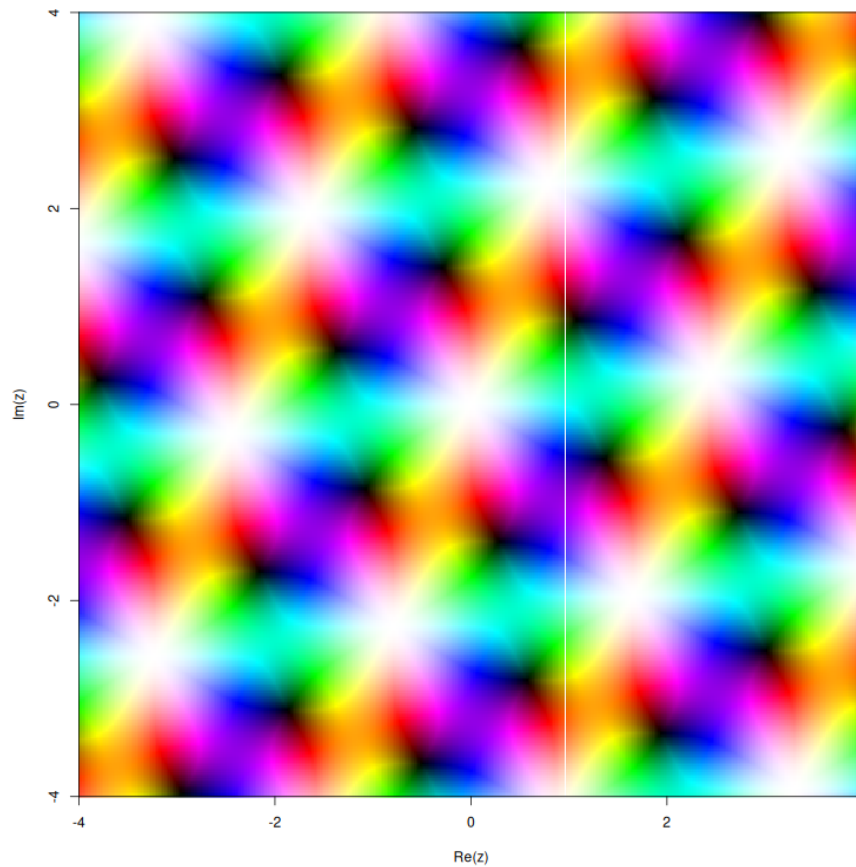
Figure 3: Visualization of \wp(z, 1, 1+2i) using the scheme of Thaller (1998): white corresponds to a pole, black to a zero, and full saturation to |\wp(z)| = 1 . The poles of \wp(z) occur on a regular lattice, and the zeros on two shifted lattices. Note how each of the poles is surrounded by two cycles of hue, indicating that they are of second order; and each of the zeros is surrounded by one cycle of hue, indicating that they are simple roots
