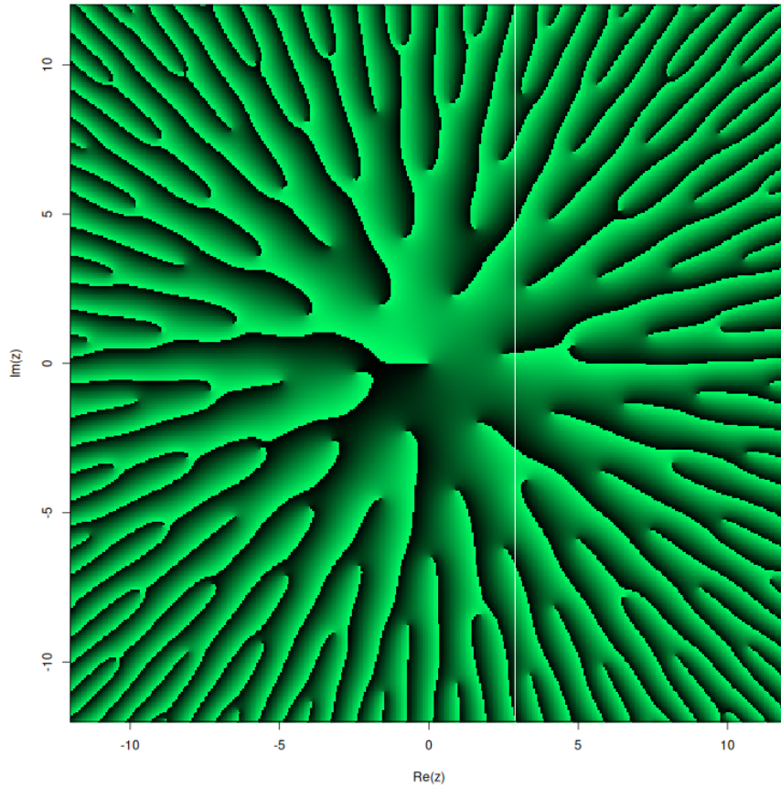
Figure 4: Visualization of f = \sigma(z, 1, 1 + 2i) using view() ; colour indicates \text{Arg}(f) . Thus points at which f(z) is on the negative real axis, that is \{z: f(z) \in \mathbb{R}^-\} , are visible as discontinuities of (colourimetric) value. These discontinuities are semi-infinite; note that the zeros of f occur, at the (finite) end of each line, on a regular lattice. As |z| increases, each discontinuity threads its way through an increasing number of other discontinuities and zeros, and the spacing between the discontinuities becomes less and less
