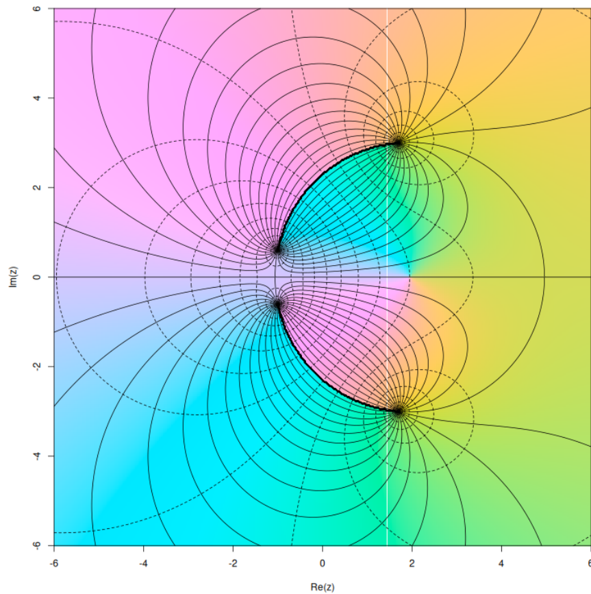
Figure 8: Potential flow in on the complex plane: two sources and two sinks, all of equal strength. Solid lines denote streamlines, dotted lines equipotentials; colour scheme uses the hc1() system: hue varies with the argument, and chrominance varies with the modulus, of the potential. There is no flux between the lower and the upper half plane, but there is flux out of, and in to, the diagram. Note the stagnation point at approximately 5 + 0i
