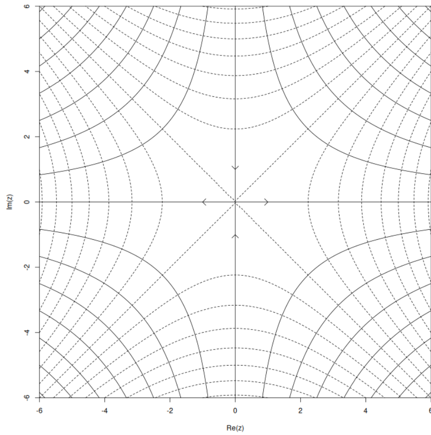
Figure 7: Potential flow on the complex plane: field corresponding to the function w(z) = z^2 . Solid lines represent streamlines and dotted lines represent equipotentials; these intersect at right angles. Note stagnation point at the origin
