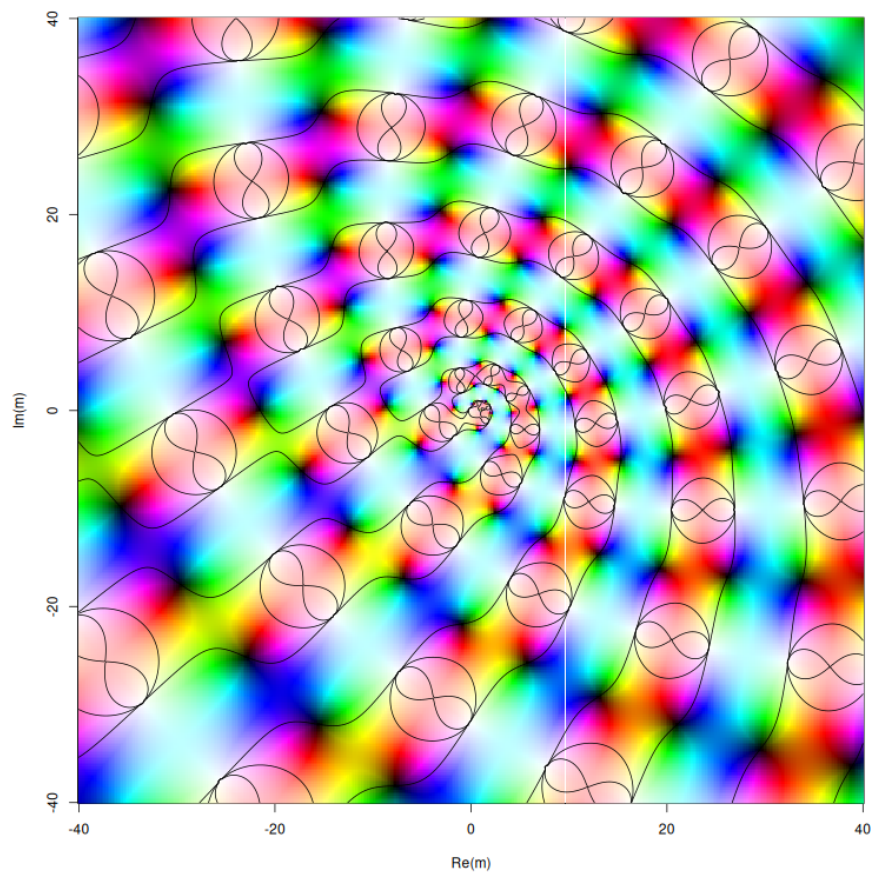
Figure 6: Jacobi's "sn" function using the elliptic package. Here, f = \text{sn}(5 - 2i, m) is visualized, with background utilizing Thaller's scheme, and contours of equal \text{Re}(f) at three selected values shown as black lines. Note the aperiodic arrangement of poles (white areas) and zeros (black areas)
