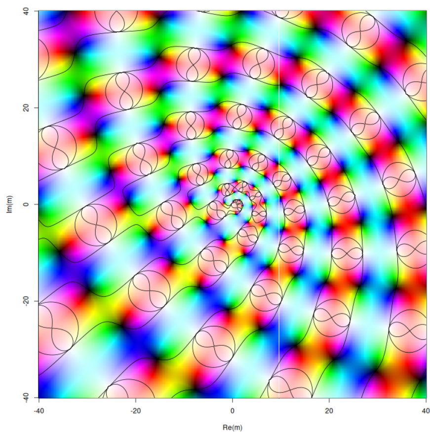
Figure 6: Jacobi's "sn" function using the elliptic package. Here, f = \operatorname{sn}(5 - 2i, m) is visualized, with background utilizing Thaller's scheme, and contours of equal \operatorname{Re}(f) at three selected values shown as black lines. Note the aperiodic arrangement of poles (white areas) and zeros (black areas)
